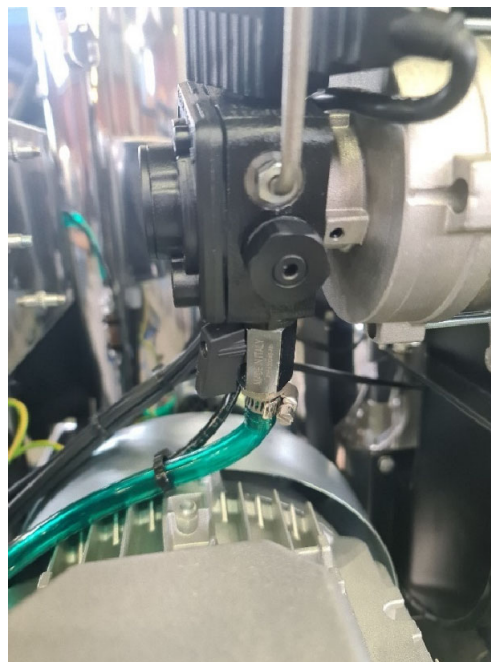
Ball valve for diesel fuel supply interruption
