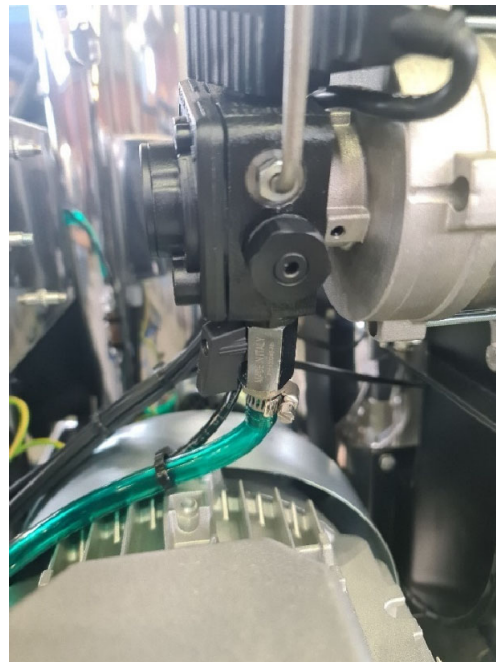
Ball valve for diesel fuel supply interruption
