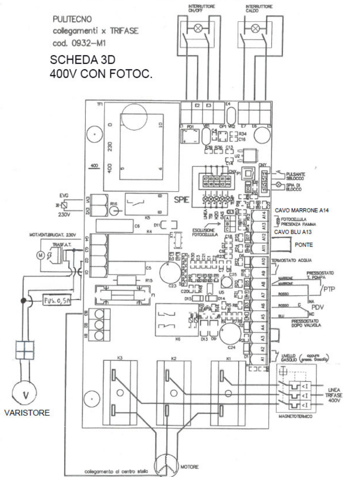
CIRCUIT BOARD DIAGRAM 400V 7,5 HP MOTORS
